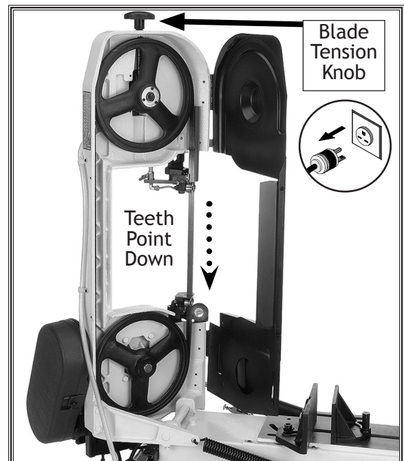
Figure 39. Open blade guard door.
